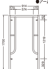
鳥居型建枠 A-3055A (900SJ)
